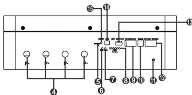
Terminal view
