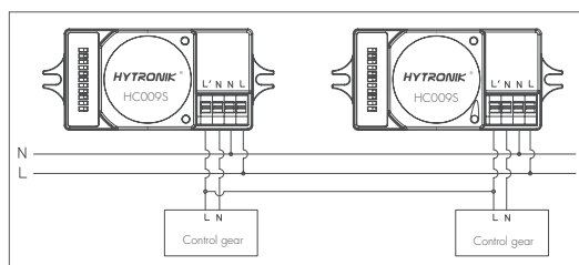
Wiring diagram for condominium function:
