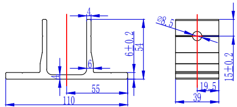
Adjustable front foot adjustment lever
