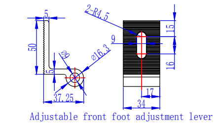
Adjustable front foot adjustment lever
