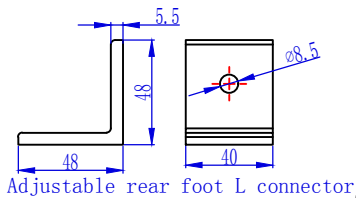
Adjustable rear foot L connector
