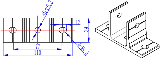
Adjustable front and rear foot base
